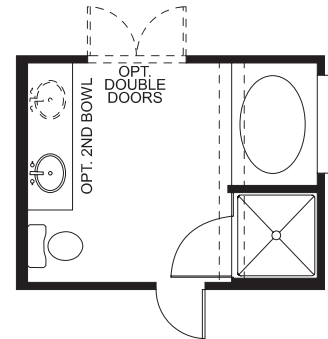
ALTERNATE OWNER'S BATH
