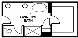
OPTIONAL LUXURY OWNER'S BATH
