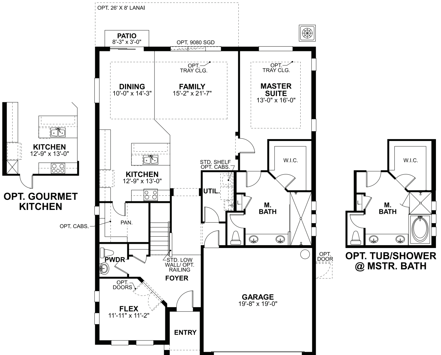
FIRST FLOOR
