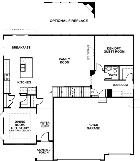
FIRST FLOOR ELEVATION A
