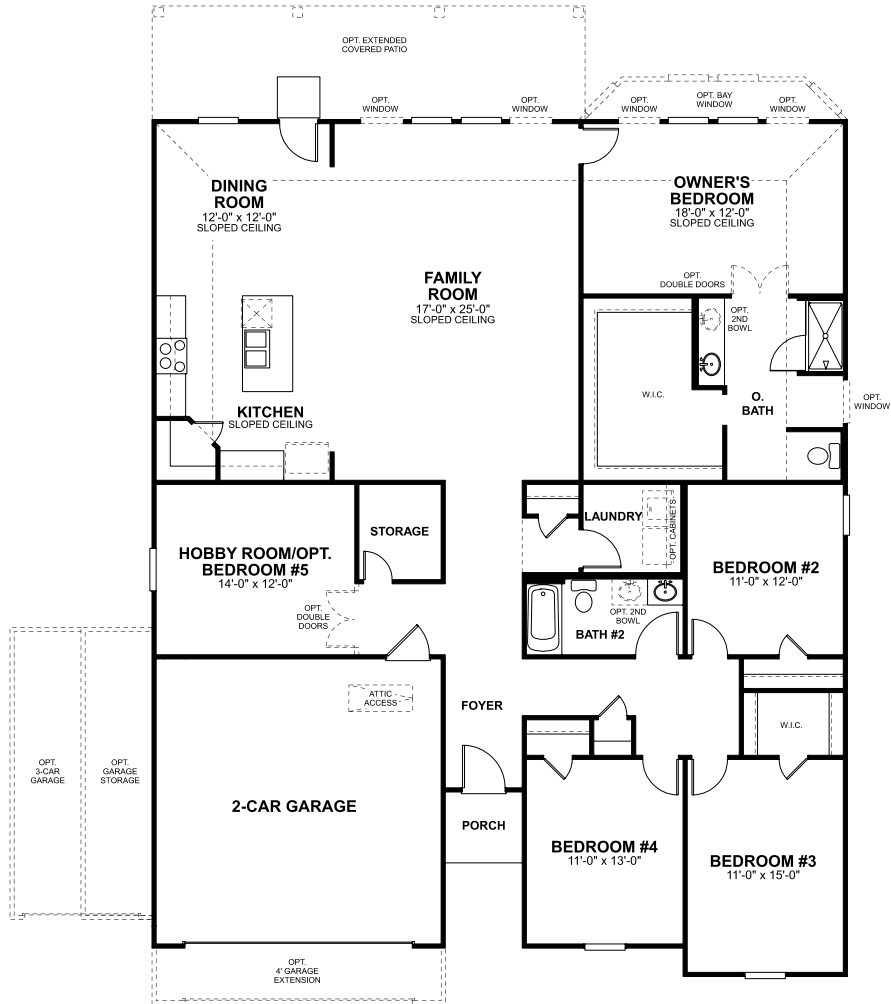
FIRST FLOOR
