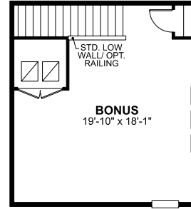
OPT. SECOND FLOOR
