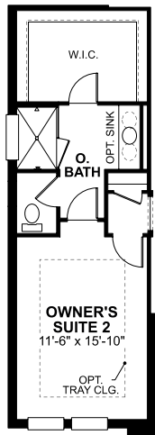
OPT. OWNER'S SUITE 2 I.L.O. BEDROOM 2
