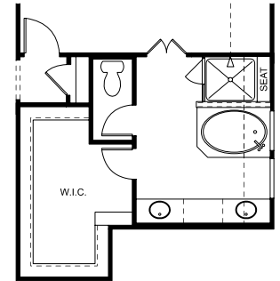
OPTIONAL LUXURY OWNER'S BATH DROP-IN TUB
