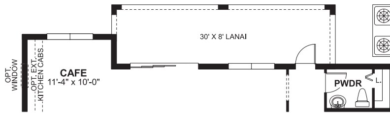
OPT. 30' X 8' LANAI W/ 9' SGD & DOUBLE CAFE WINDOW
