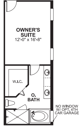
OPT. OWNER'S SUITE 2 W/ TUB AND SHOWER ILO TANDEM GARAGE
