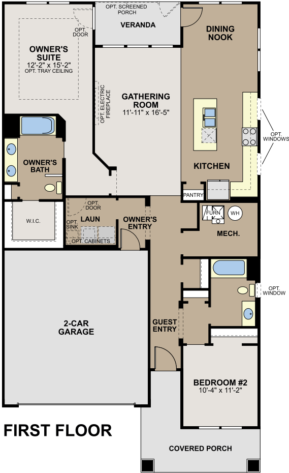
OPTIONAL 6' VERANDA EXTENSION
