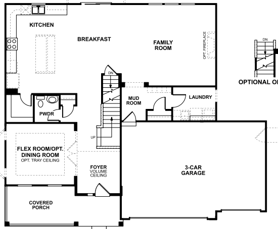
MAIN FLOOR ELEVATION CLASSICAL
