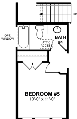
OPTIONAL BEDROOM #5/BATH #4
